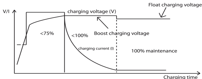
Fig. 2: Charging chart (basic curve)
