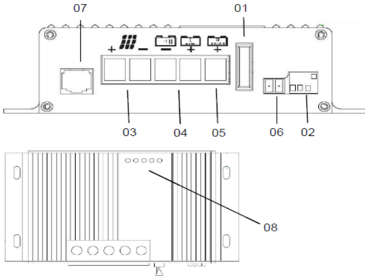
Fig 1: Device elements
